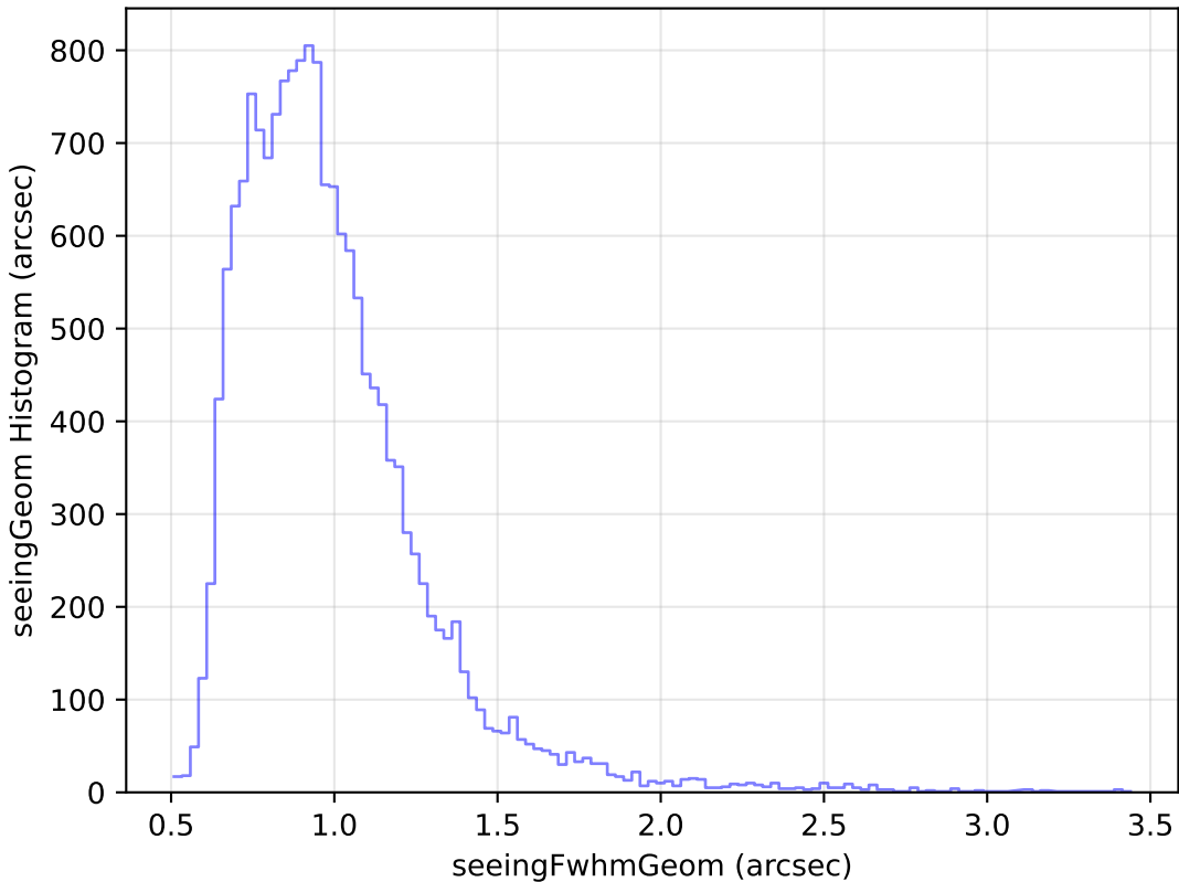
weather_cloudso14v3.4_10yrs Yr 1 u band: seeingGeom Histogram
