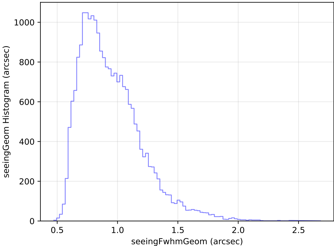
weather_cloudso14v3.4_10yrs Yr 1 g band: seeingGeom Histogram
