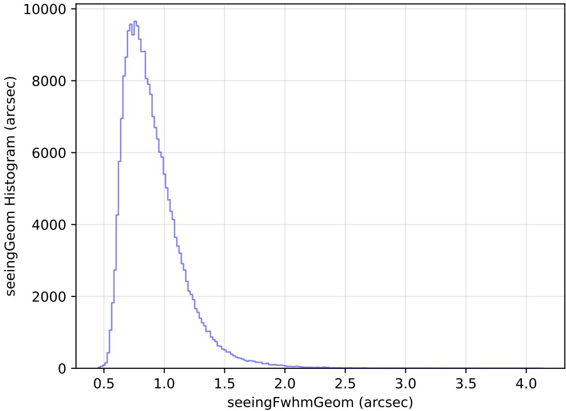
weather_cloudso14v3.4_10yrs Yr 1 all bands: seeingGeom Histogram
