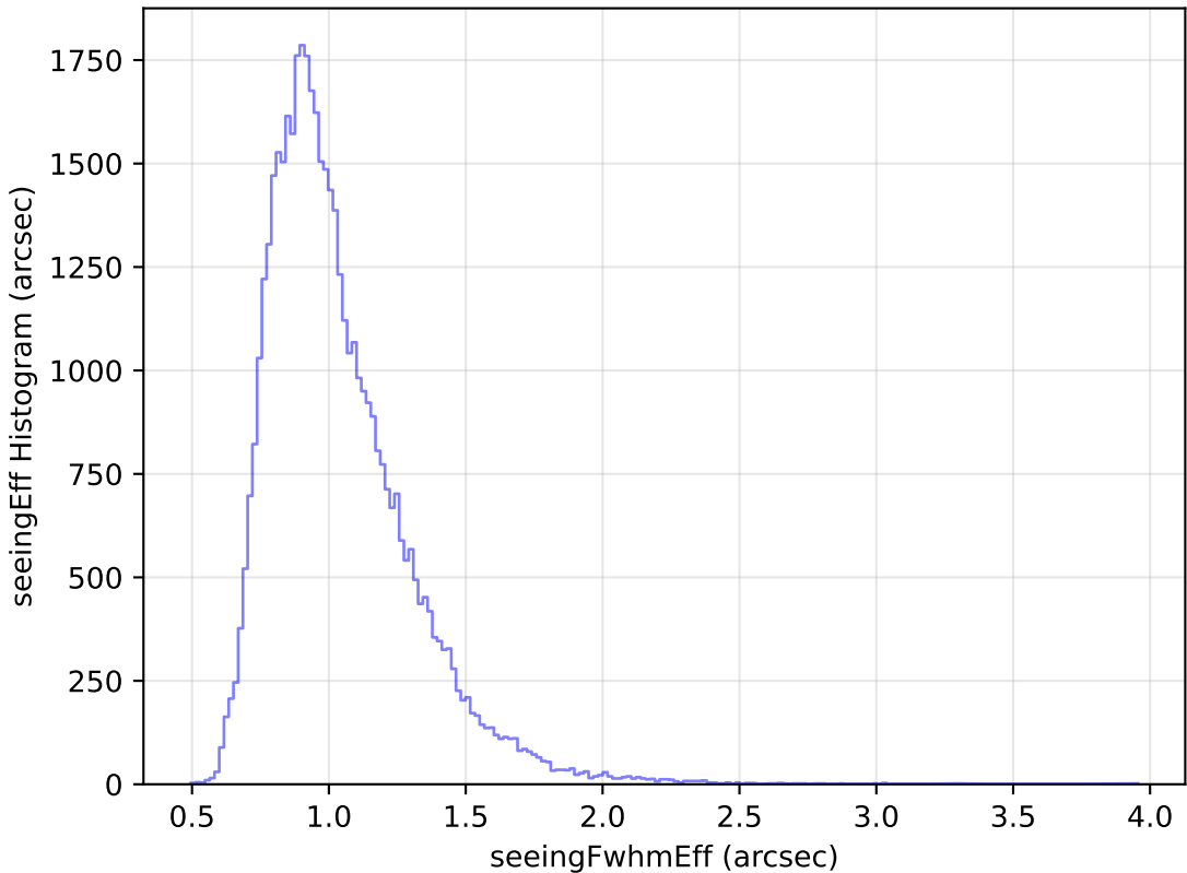
weather_cloudso14v3.4_10yrs Yr 1 y band: seeingEff Histogram
