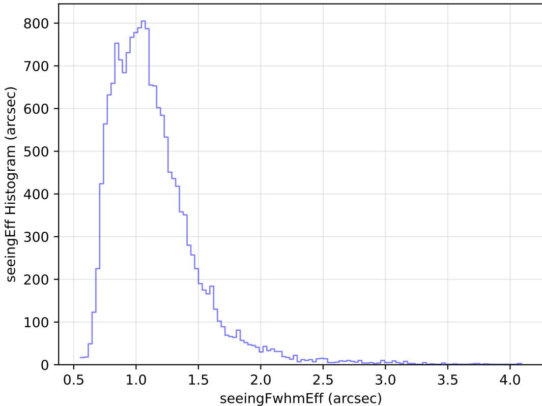
weather_cloudso14v3.4_10yrs Yr 1 u band: seeingEff Histogram
