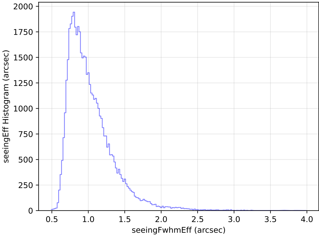
weather_cloudso14v3.4_10yrs Yr 1 r band: seeingEff Histogram
