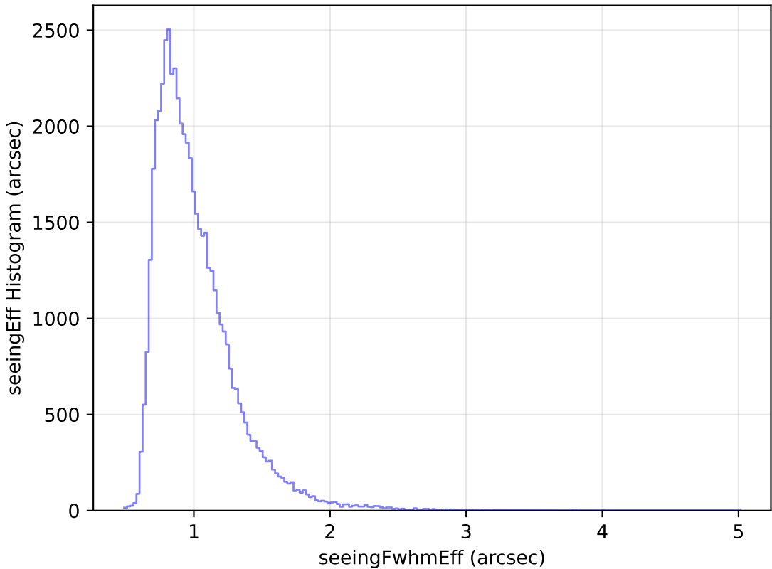
weather_cloudso14v3.4_10yrs Yr 1 i band: seeingEff Histogram
