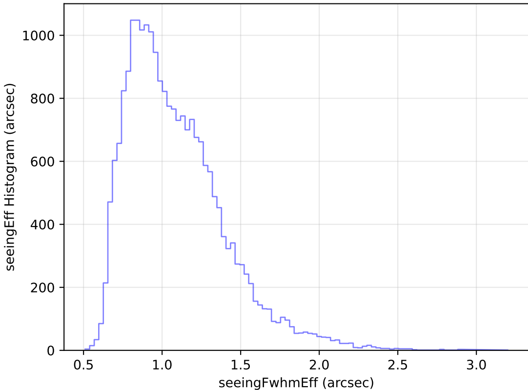
weather_cloudso14v3.4_10yrs Yr 1 g band: seeingEff Histogram
