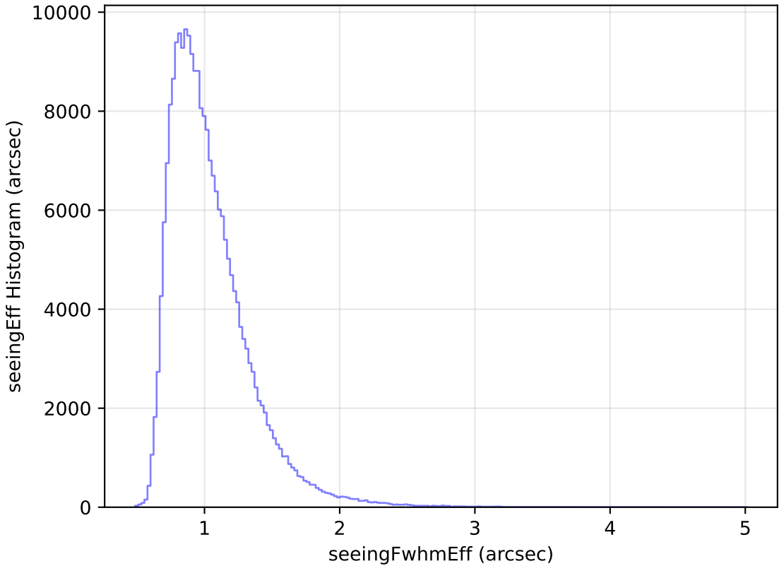
weather_cloudso14v3.4_10yrs Yr 1 all bands: seeingEff Histogram
