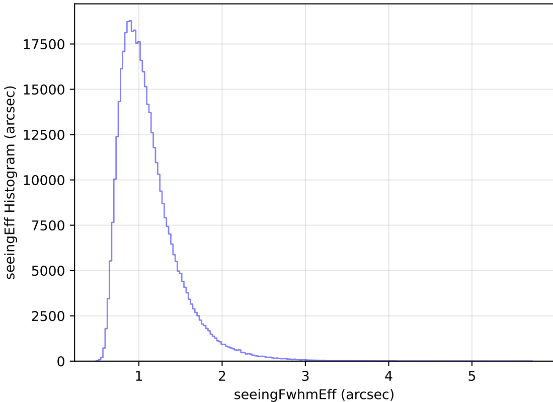
weather_cloudso14v3.4_10yrs WFD z band: seeingEff Histogram
