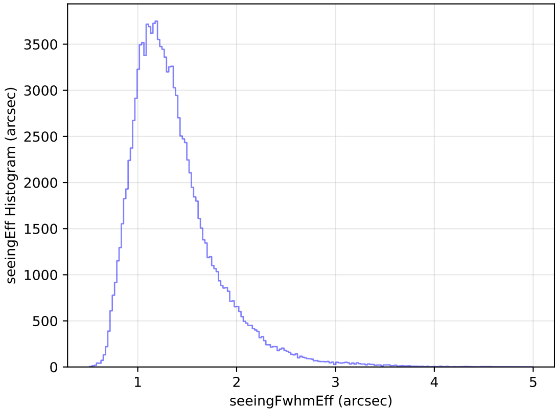
weather_cloudso14v3.4_10yrs WFD u band: seeingEff Histogram
