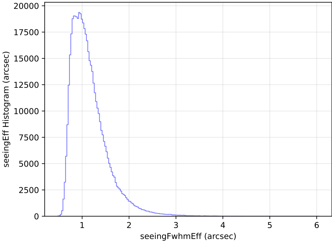
weather_cloudso14v3.4_10yrs WFD r band: seeingEff Histogram
