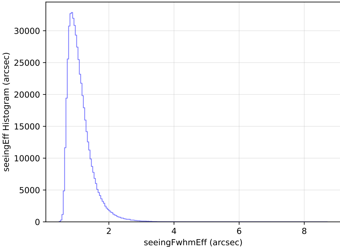
weather_cloudso14v3.4_10yrs WFD i band: seeingEff Histogram
