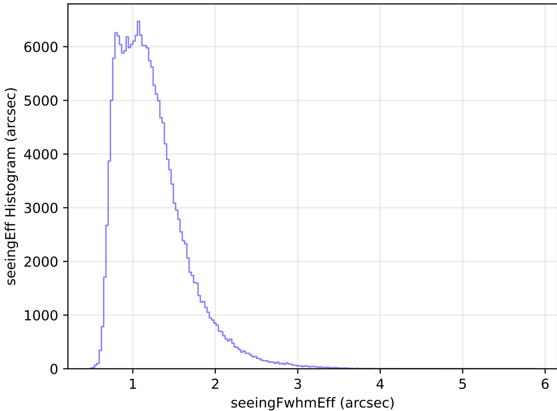
weather_cloudso14v3.4_10yrs WFD g band: seeingEff Histogram
