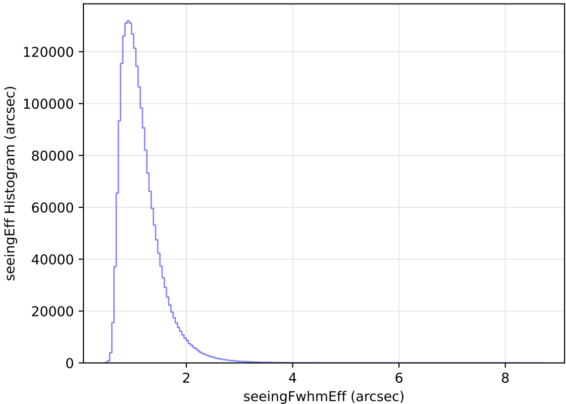
weather_cloudso14v3.4_10yrs WFD all bands: seeingEff Histogram
