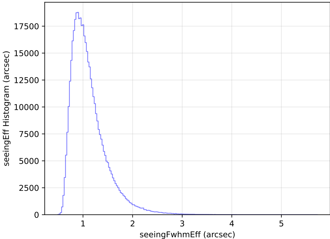
weather_cloudso14v3.4_10yrs All sky z band: seeingEff Histogram
