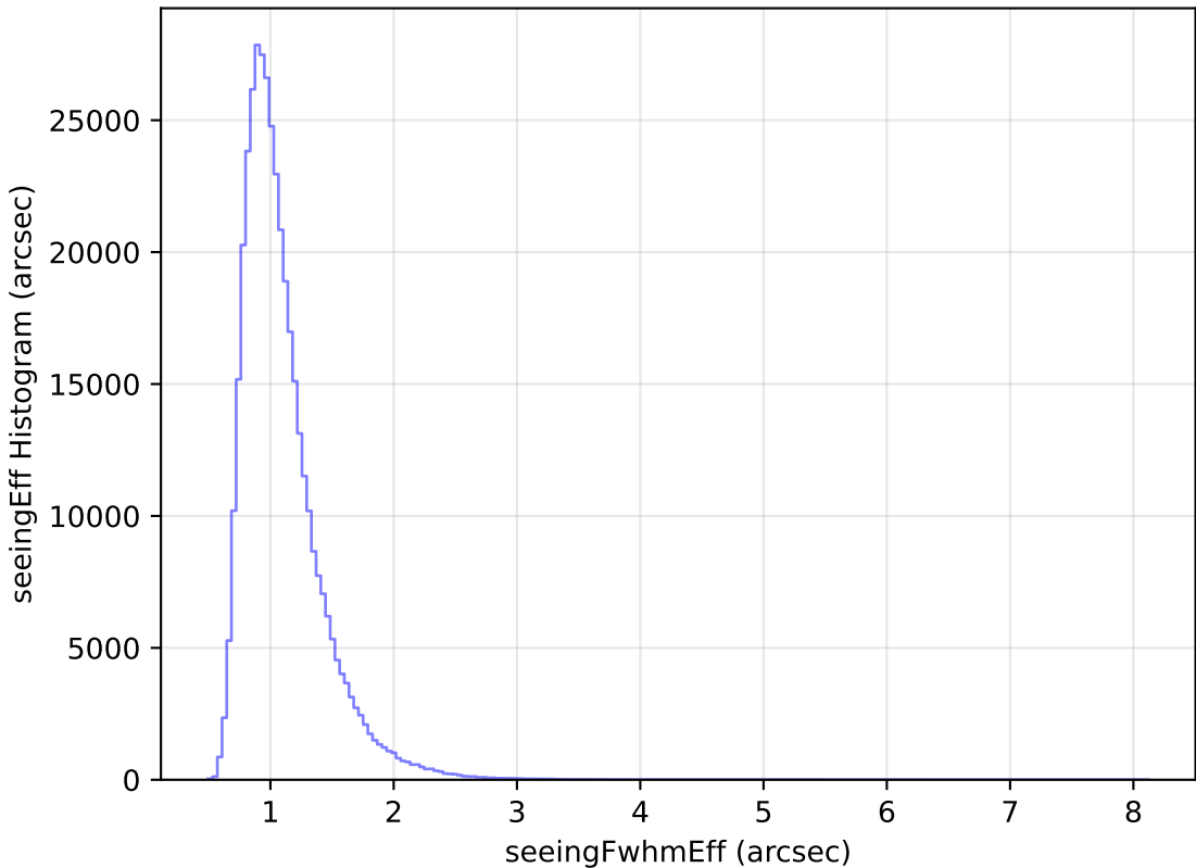
weather_cloudso14v3.4_10yrs All sky y band: seeingEff Histogram
