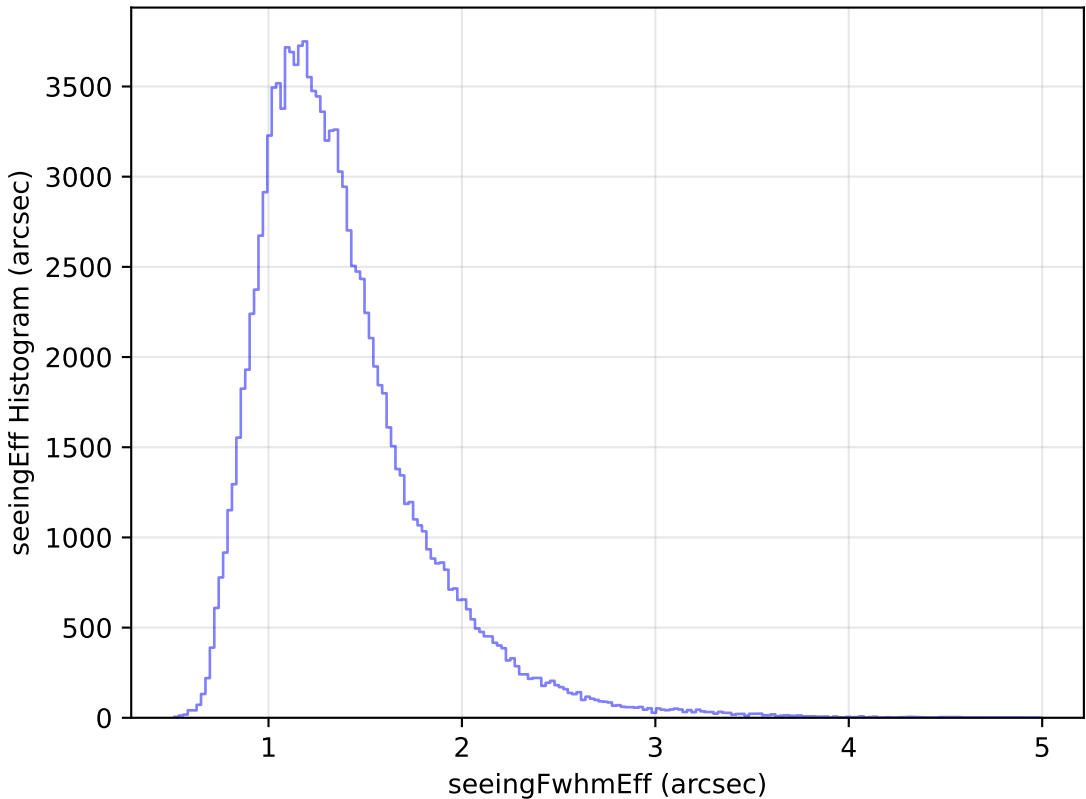
weather_cloudso14v3.4_10yrs All sky u band: seeingEff Histogram
