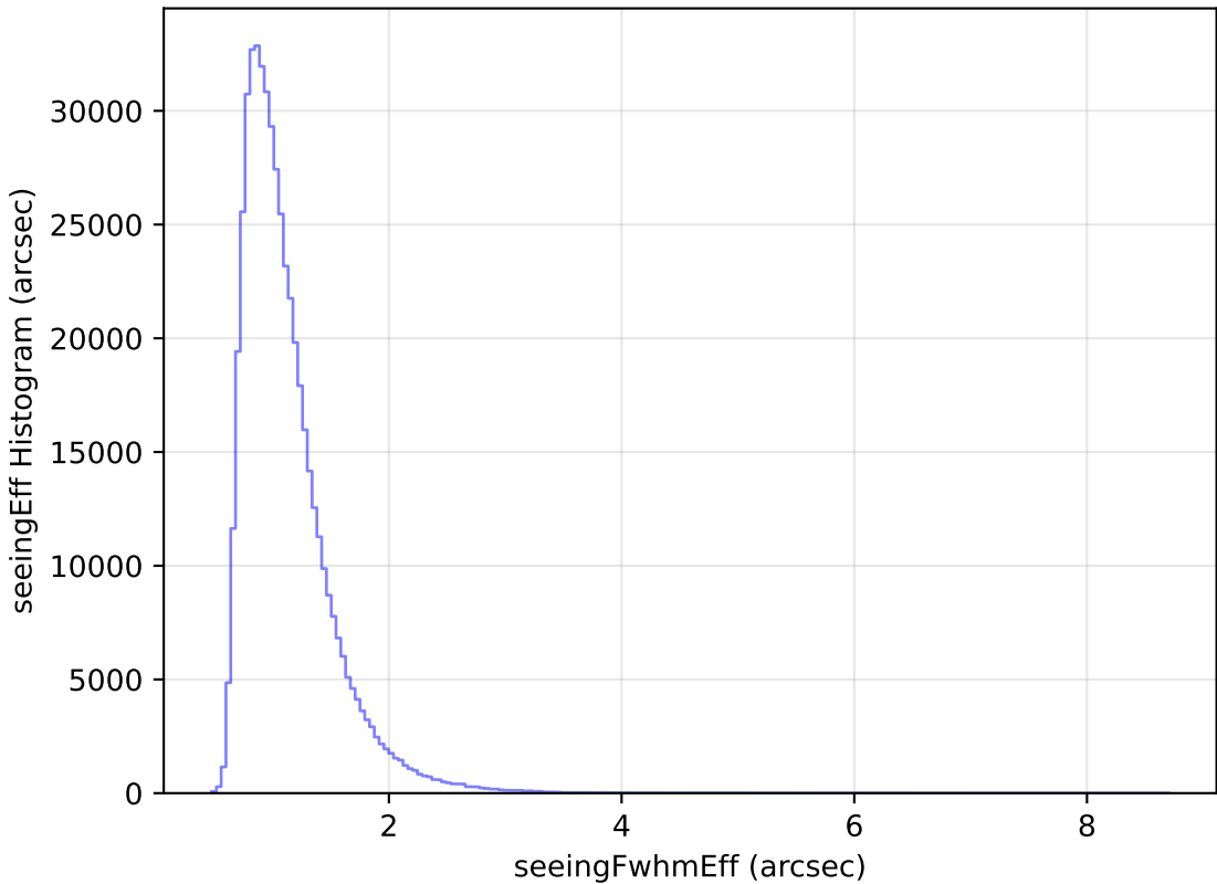
weather_cloudso14v3.4_10yrs All sky i band: seeingEff Histogram
