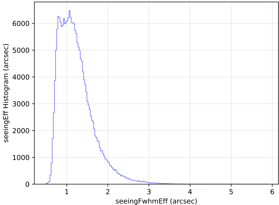
weather_cloudso14v3.4_10yrs All sky g band: seeingEff Histogram
