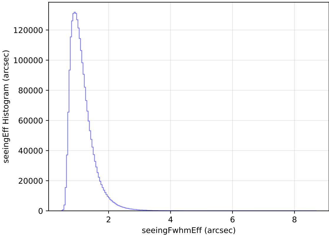
weather_cloudso14v3.4_10yrs All sky all bands: seeingEff Histogram
