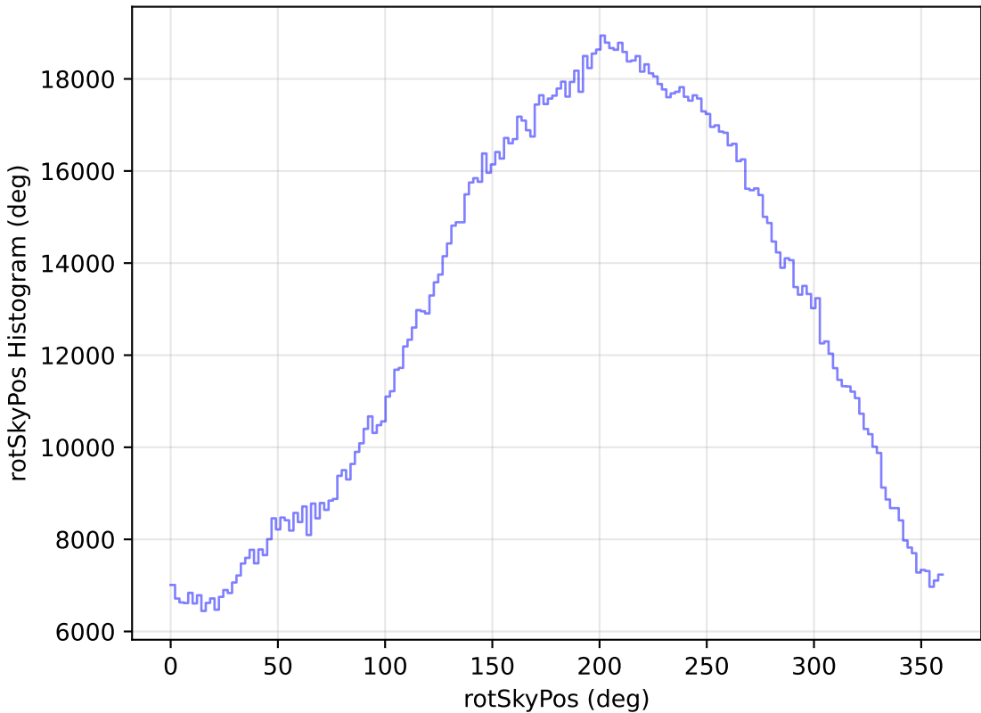
weather_cloudso14v3.4_10yrs WFD all bands: rotSkyPos Histogram
