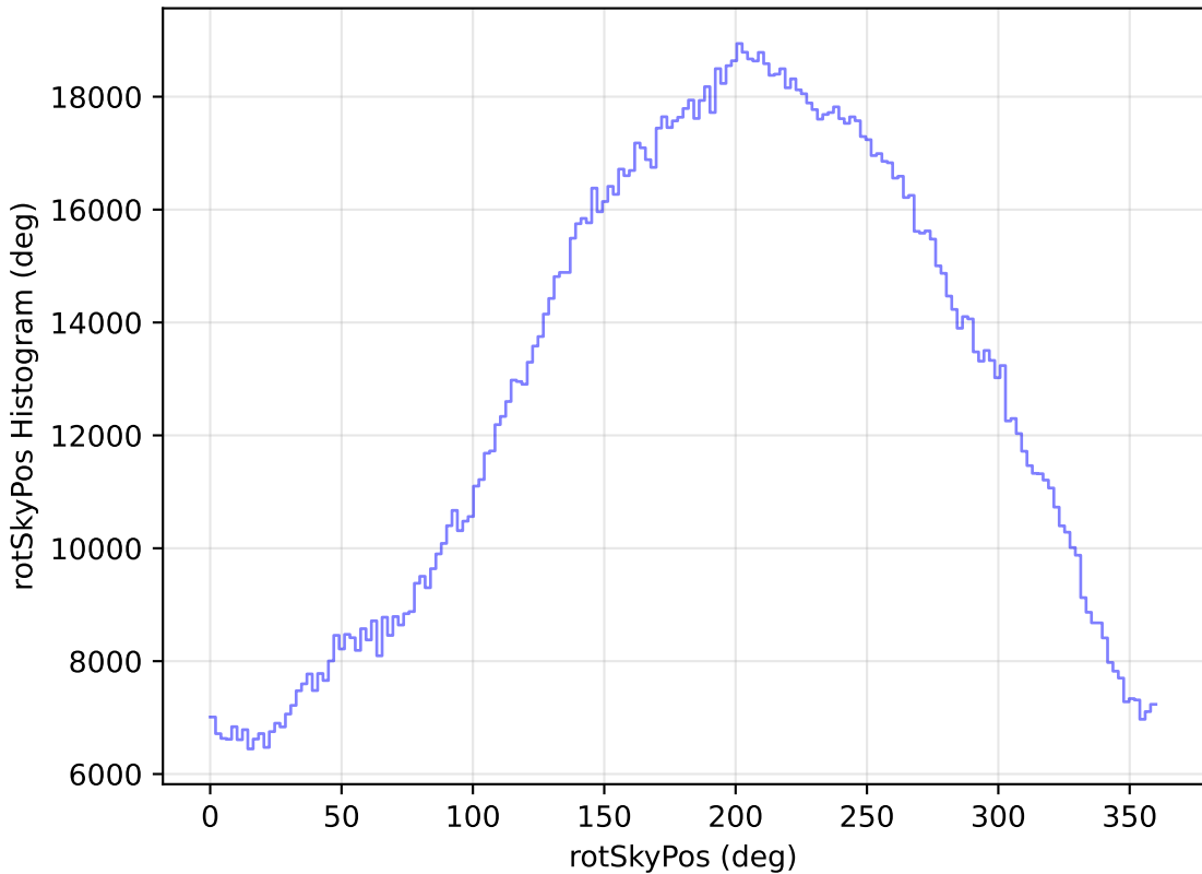
weather_cloudso14v3.4_10yrs All sky all bands: rotSkyPos Histogram
