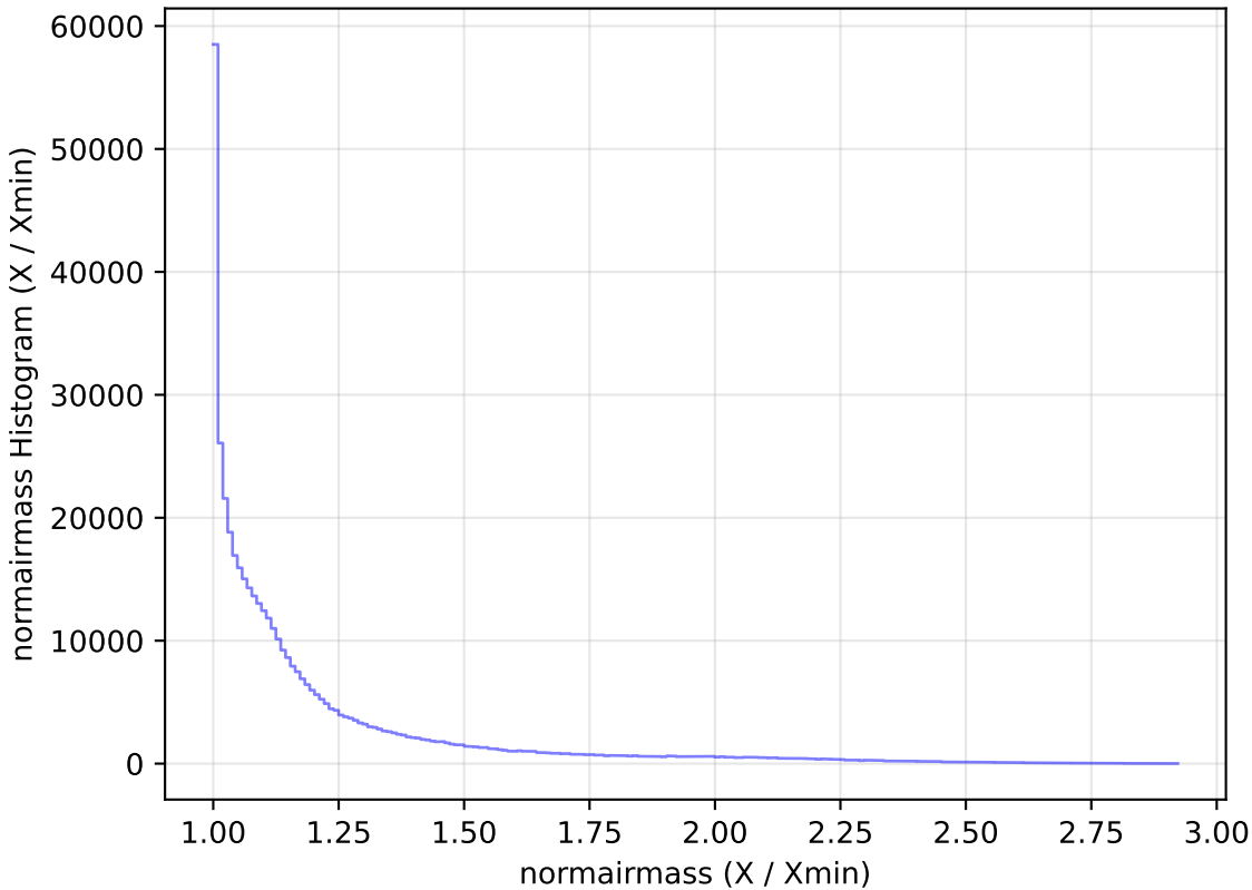
weather_cloudso14v3.4_10yrs WFD z band: normairmass Histogram
