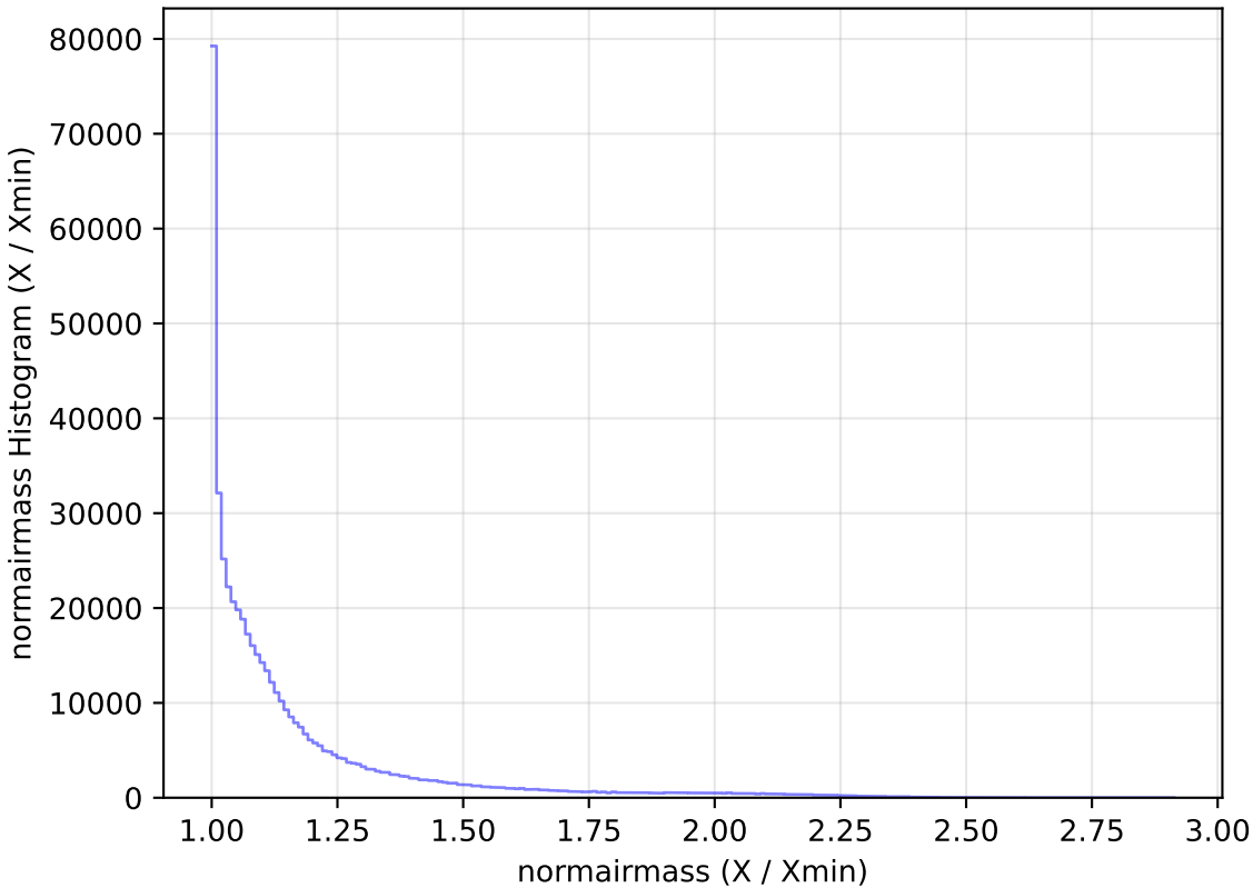
weather_cloudso14v3.4_10yrs WFD r band: normairmass Histogram
