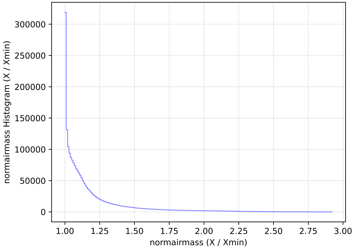
weather_cloudso14v3.4_10yrs WFD all bands: normairmass Histogram
