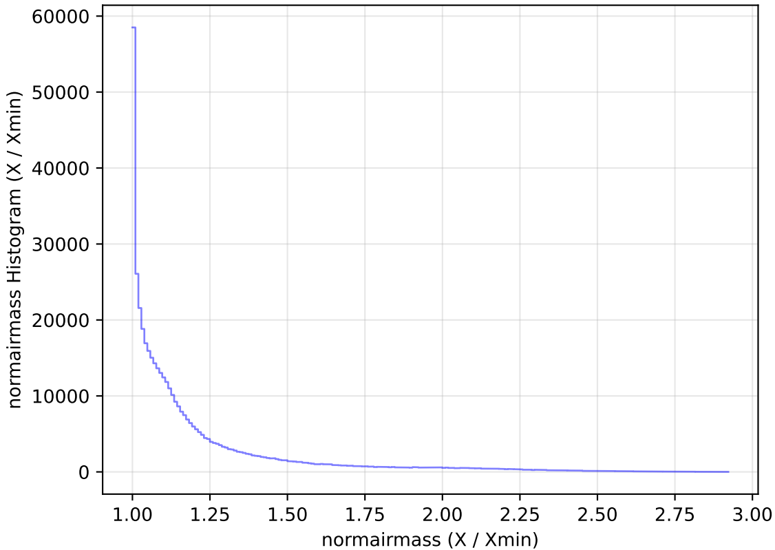
weather_cloudso14v3.4_10yrs All sky z band: normairmass Histogram
