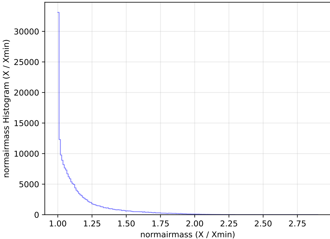
weather_cloudso14v3.4_10yrs All sky g band: normairmass Histogram
