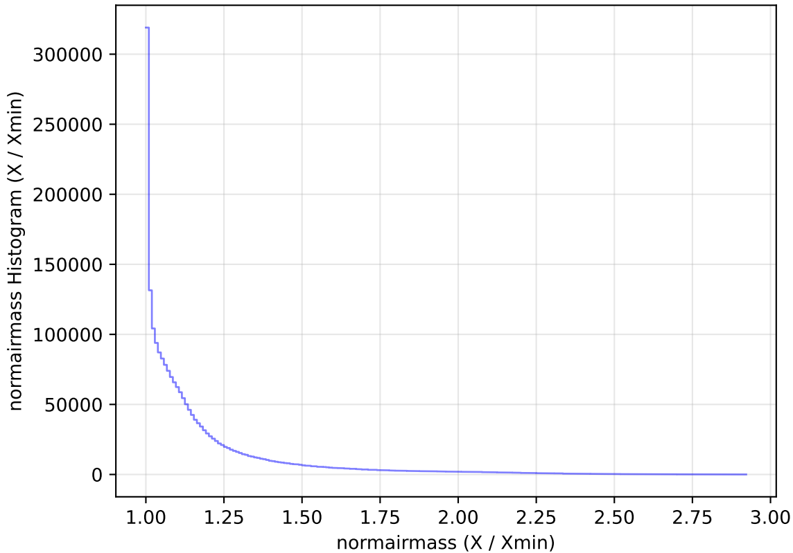
weather_cloudso14v3.4_10yrs All sky all bands: normairmass Histogram
