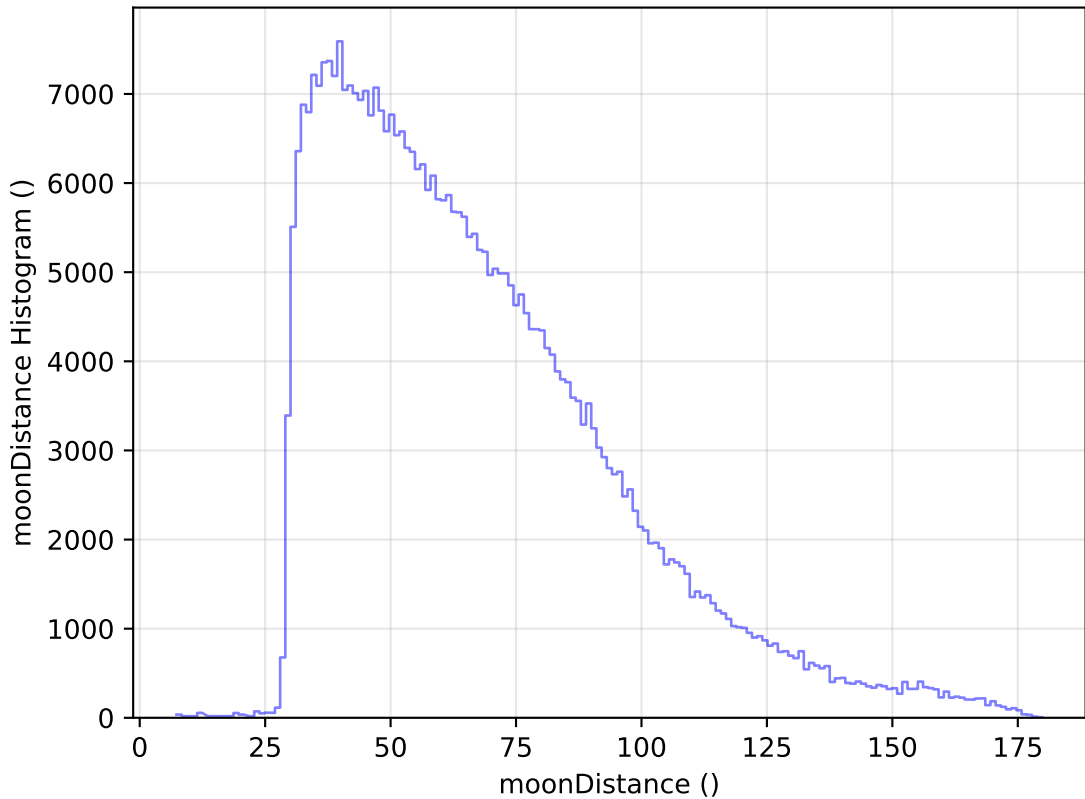
weather_cloudso14v3.4_10yrs WFD y band: moonDistance Histogram
