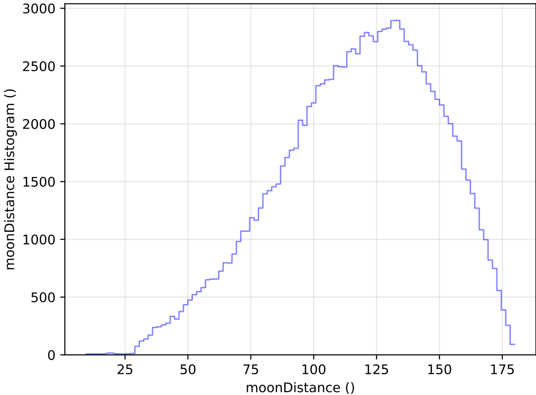
weather_cloudso14v3.4_10yrs WFD u band: moonDistance Histogram
