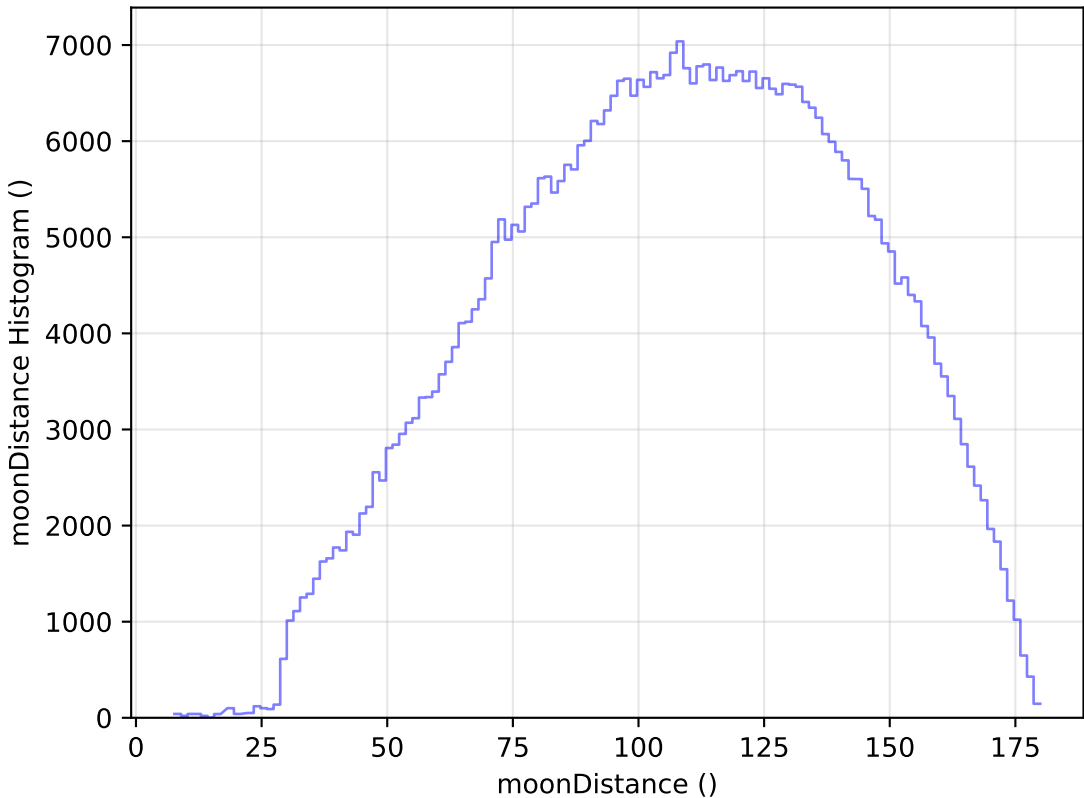
weather_cloudso14v3.4_10yrs WFD r band: moonDistance Histogram
