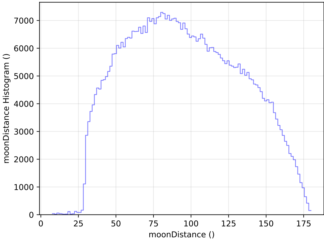
weather_cloudso14v3.4_10yrs WFD i band: moonDistance Histogram
