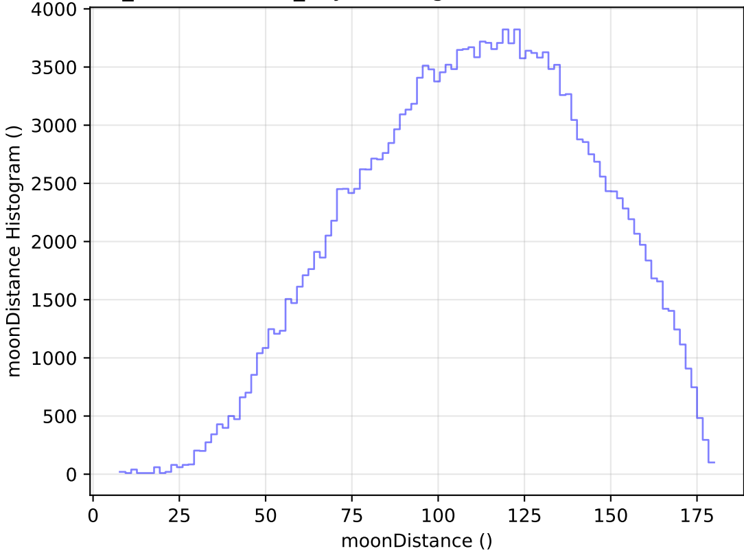
weather_cloudso14v3.4_10yrs WFD g band: moonDistance Histogram
