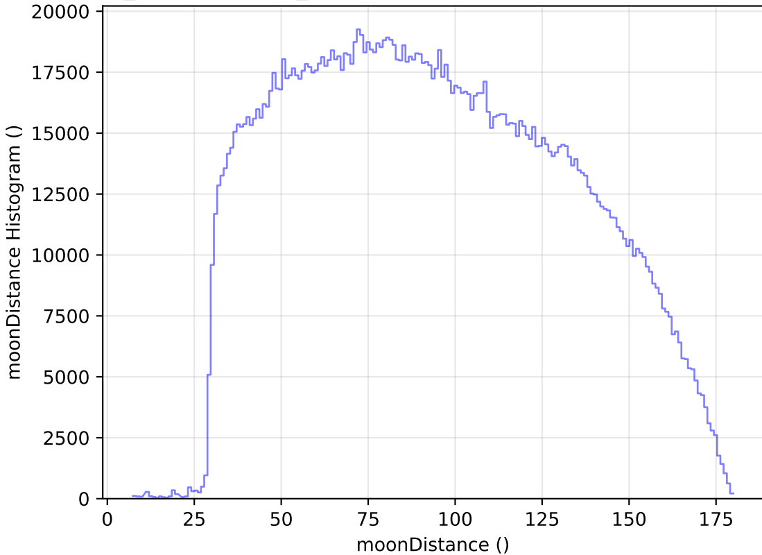
weather_cloudso14v3.4_10yrs WFD all bands: moonDistance Histogram
