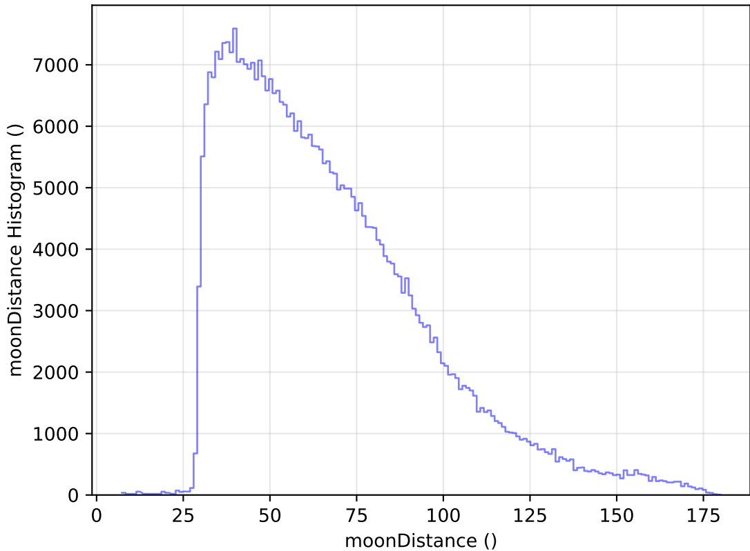
weather_cloudso14v3.4_10yrs All sky y band: moonDistance Histogram
