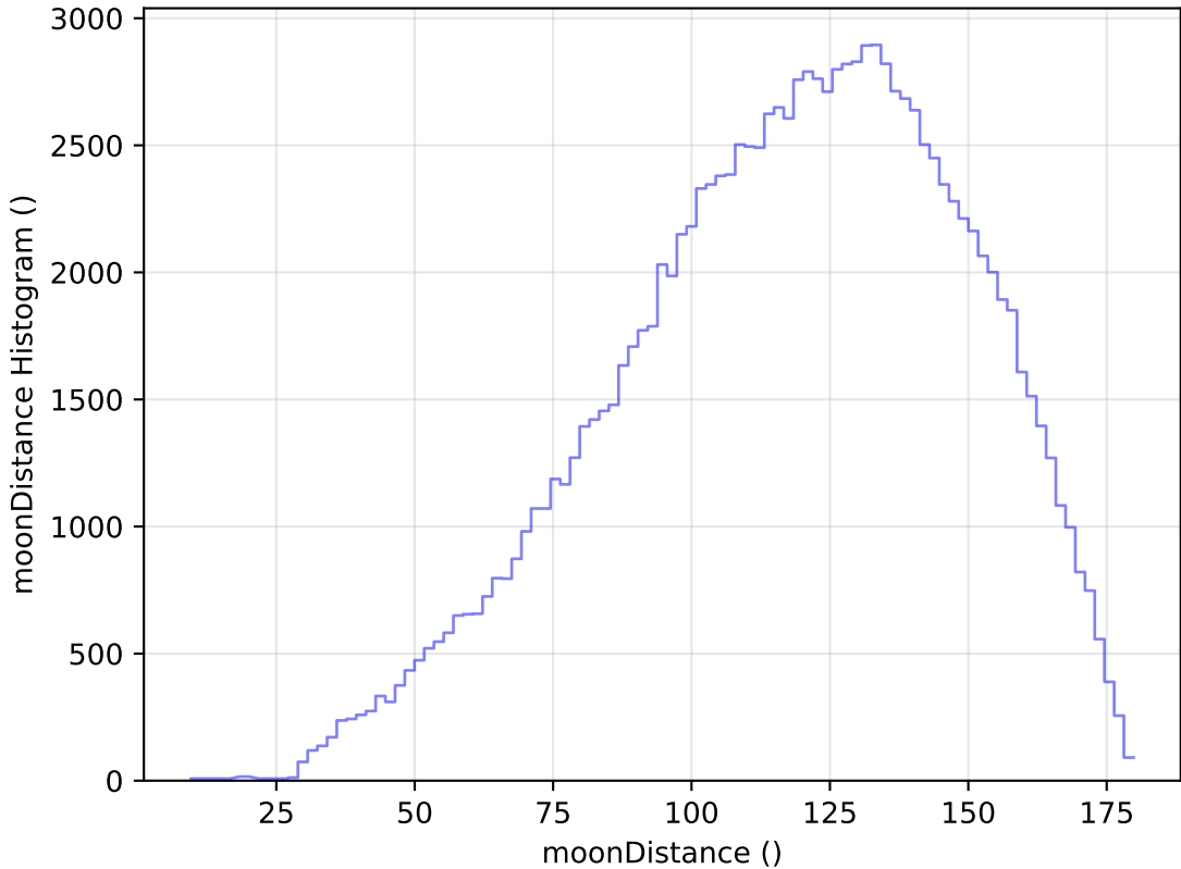
weather_cloudso14v3.4_10yrs All sky u band: moonDistance Histogram
