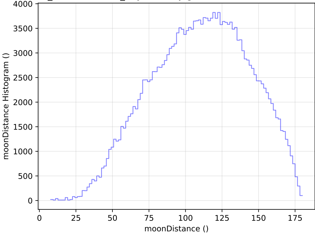
weather_cloudso14v3.4_10yrs All sky g band: moonDistance Histogram
