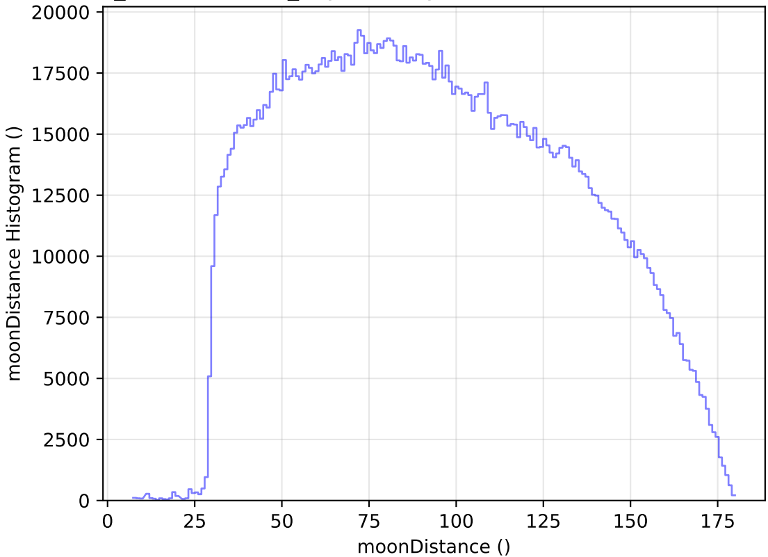
weather_cloudso14v3.4_10yrs All sky all bands: moonDistance Histogram
