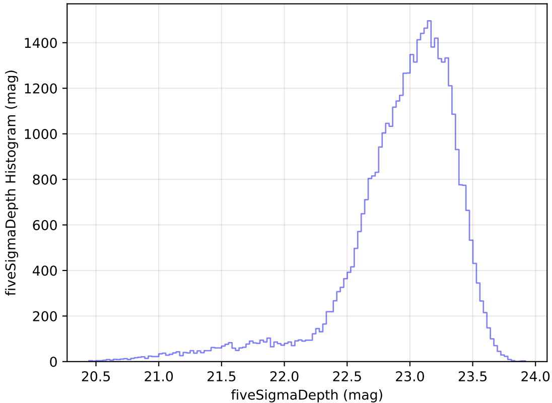
weather_cloudso14v3.4_10yrs Yr 1 z band: fiveSigmaDepth Histogram
