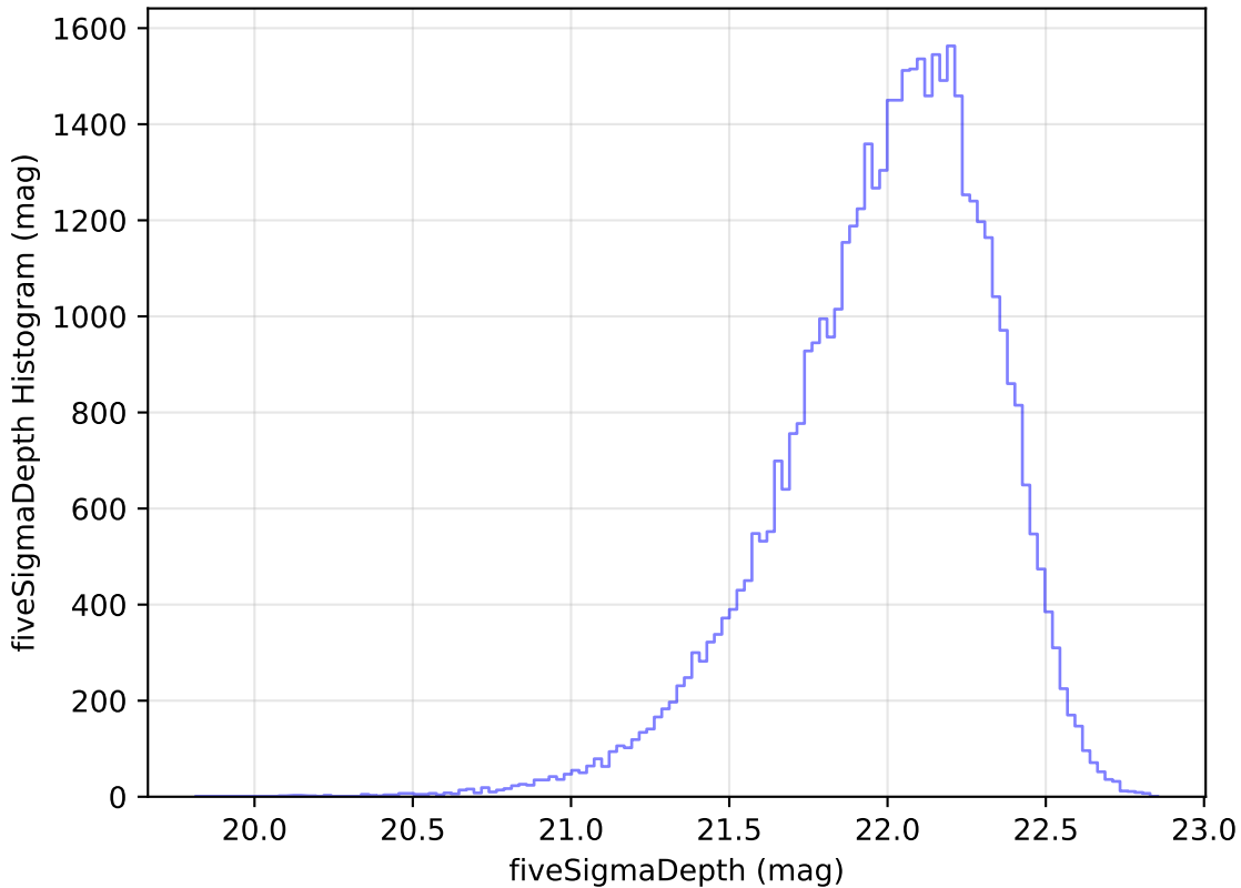
weather_cloudso14v3.4_10yrs Yr 1 y band: fiveSigmaDepth Histogram
