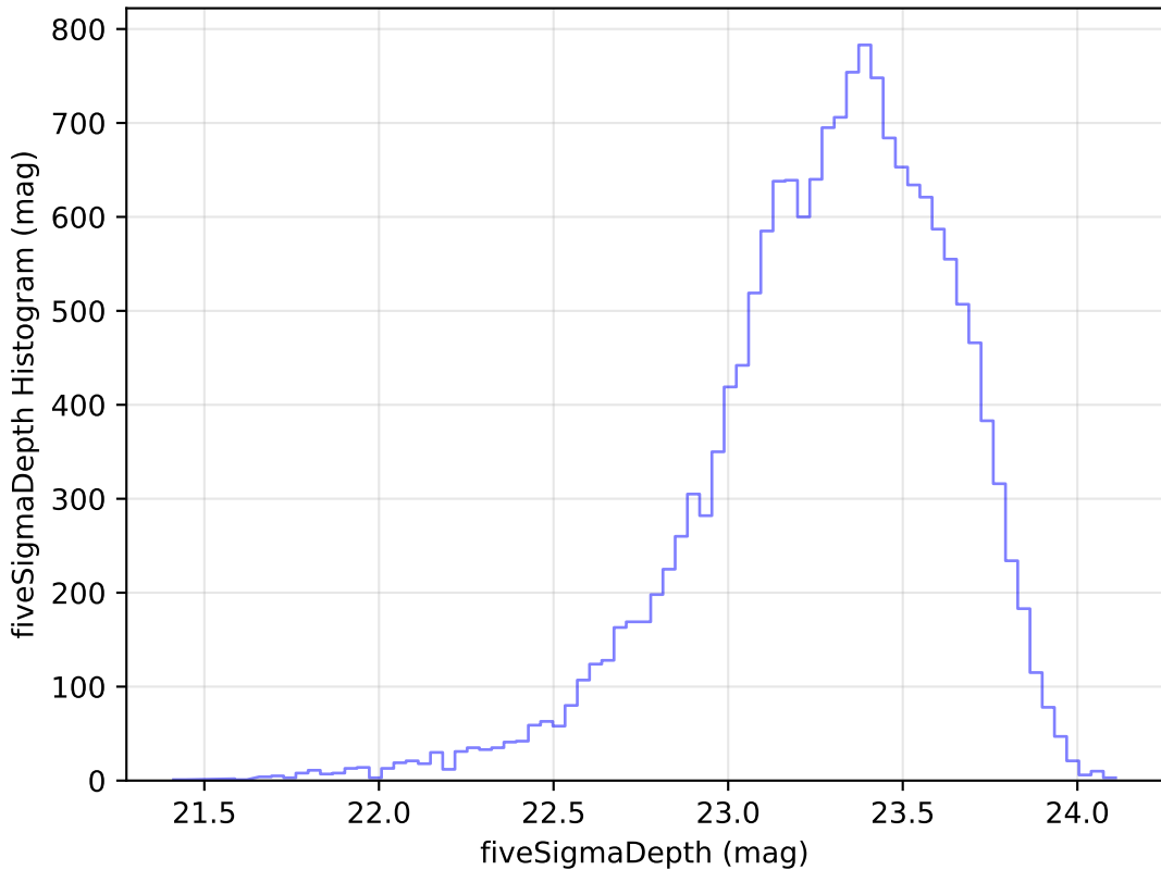
weather_cloudso14v3.4_10yrs Yr 1 u band: fiveSigmaDepth Histogram
