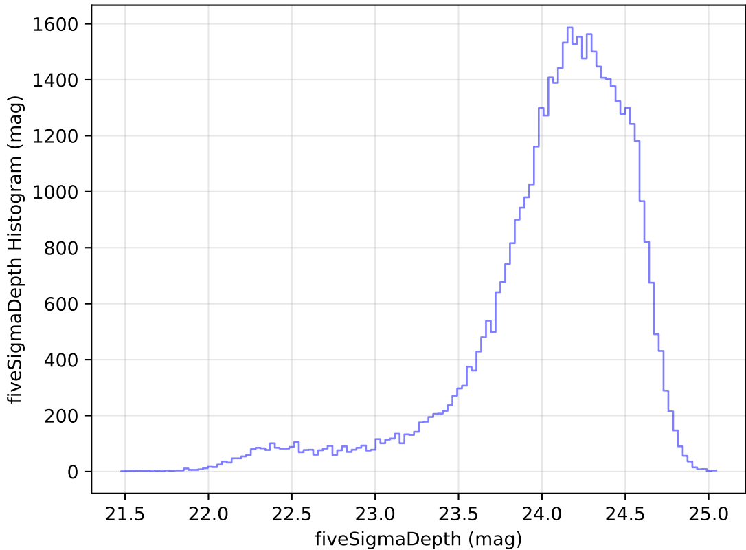
weather_cloudso14v3.4_10yrs Yr 1 r band: fiveSigmaDepth Histogram
