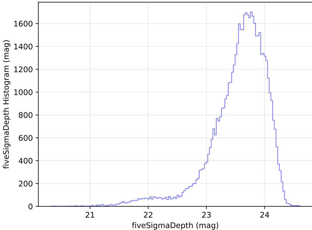
weather_cloudso14v3.4_10yrs Yr 1 i band: fiveSigmaDepth Histogram
