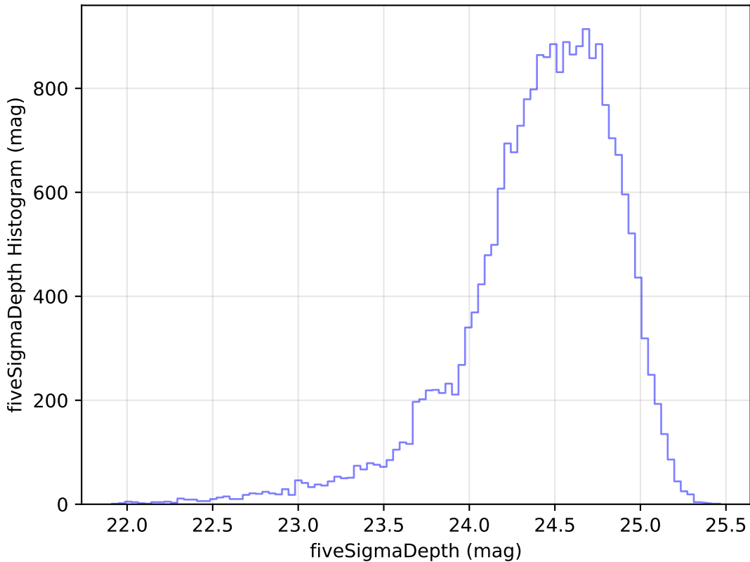
weather_cloudso14v3.4_10yrs Yr 1 g band: fiveSigmaDepth Histogram
