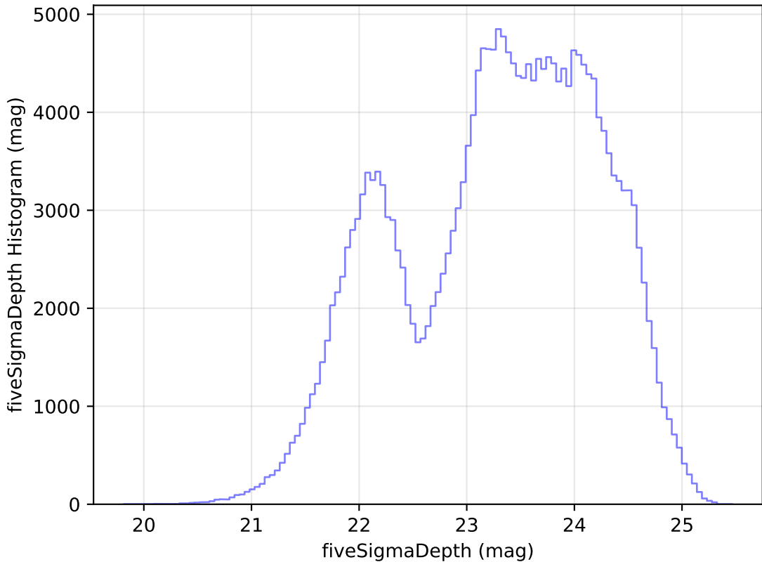
weather_cloudso14v3.4_10yrs Yr 1 all bands: fiveSigmaDepth Histogram
