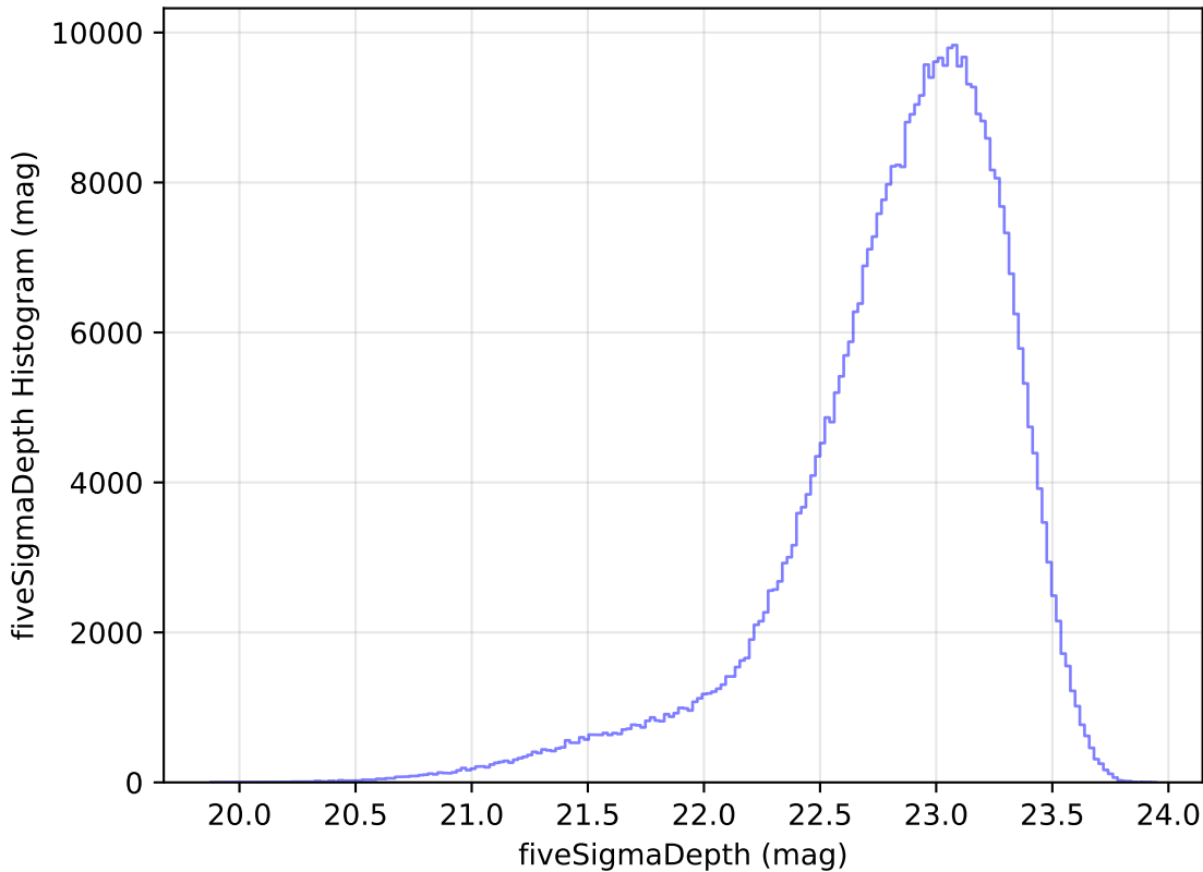
weather_cloudso14v3.4_10yrs WFD z band: fiveSigmaDepth Histogram
