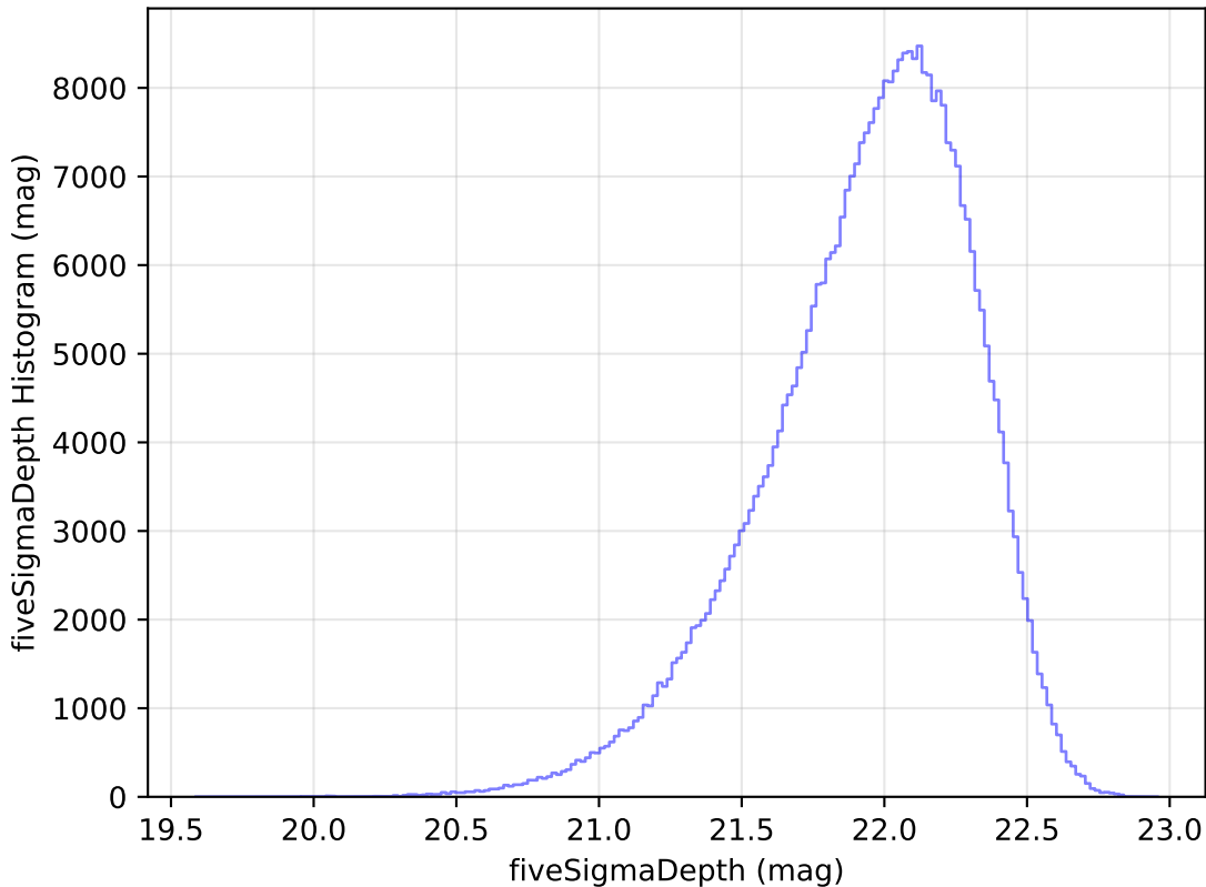
weather_cloudso14v3.4_10yrs WFD y band: fiveSigmaDepth Histogram
