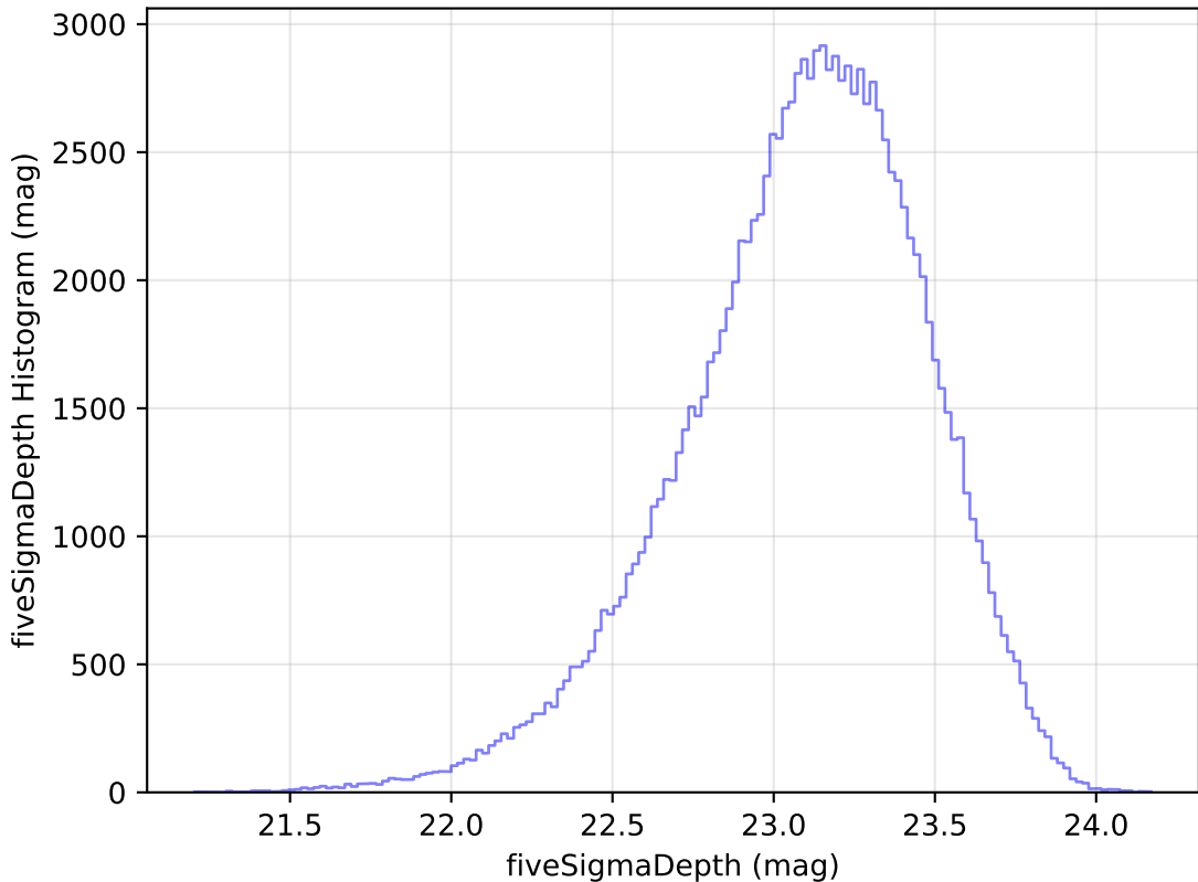
weather_cloudso14v3.4_10yrs WFD u band: fiveSigmaDepth Histogram
