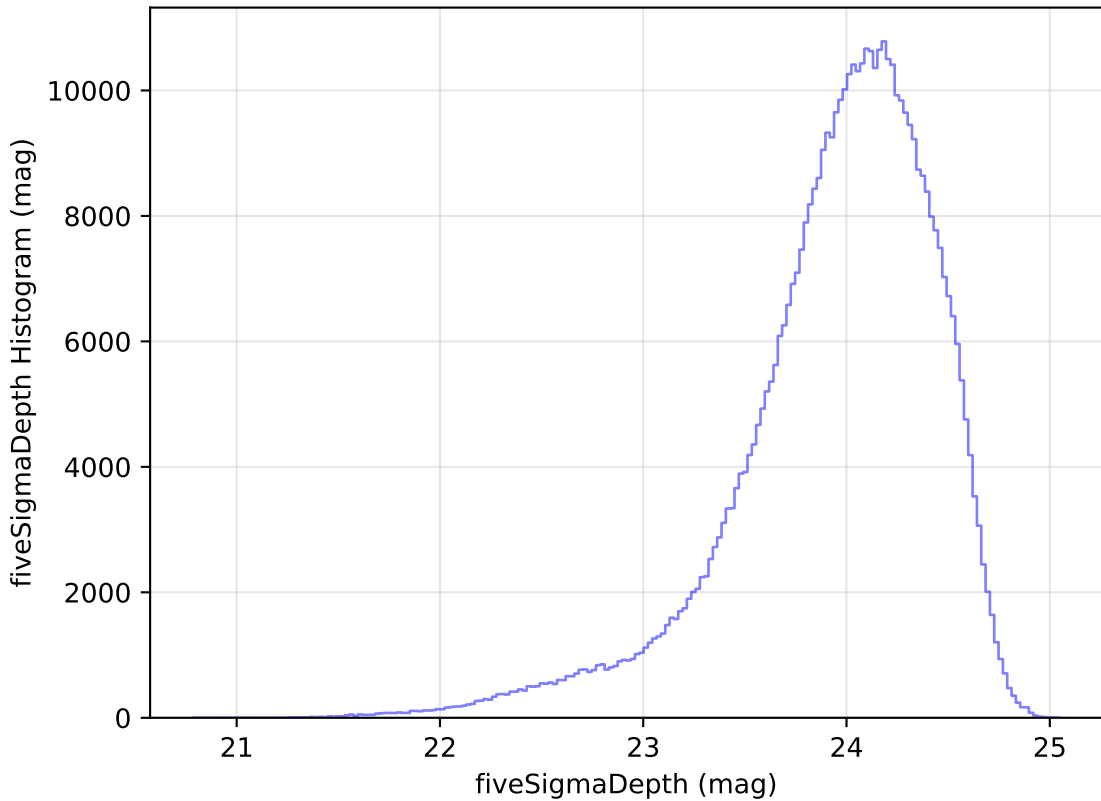
weather_cloudso14v3.4_10yrs WFD r band: fiveSigmaDepth Histogram
